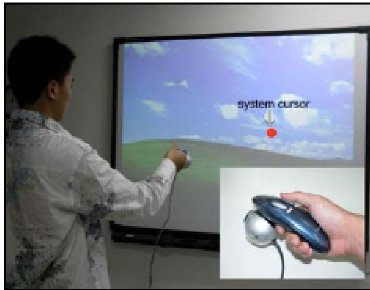
Figure 2.6: Direct Pointer uses a handheld camera to track a cursor displayed on the remote screen without relying on visual tags. (Jiang et al. , 2006)
