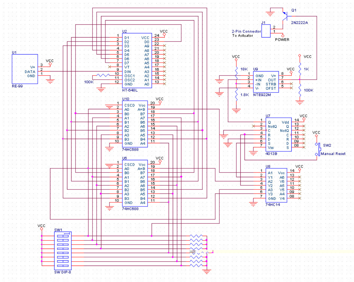
Figure A.2: The circuit diagram for the iLight.
