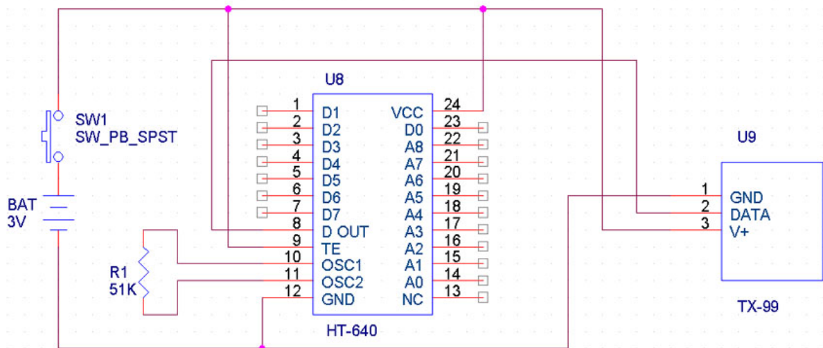
Figure A.1: The circuit diagram for the iButton.
