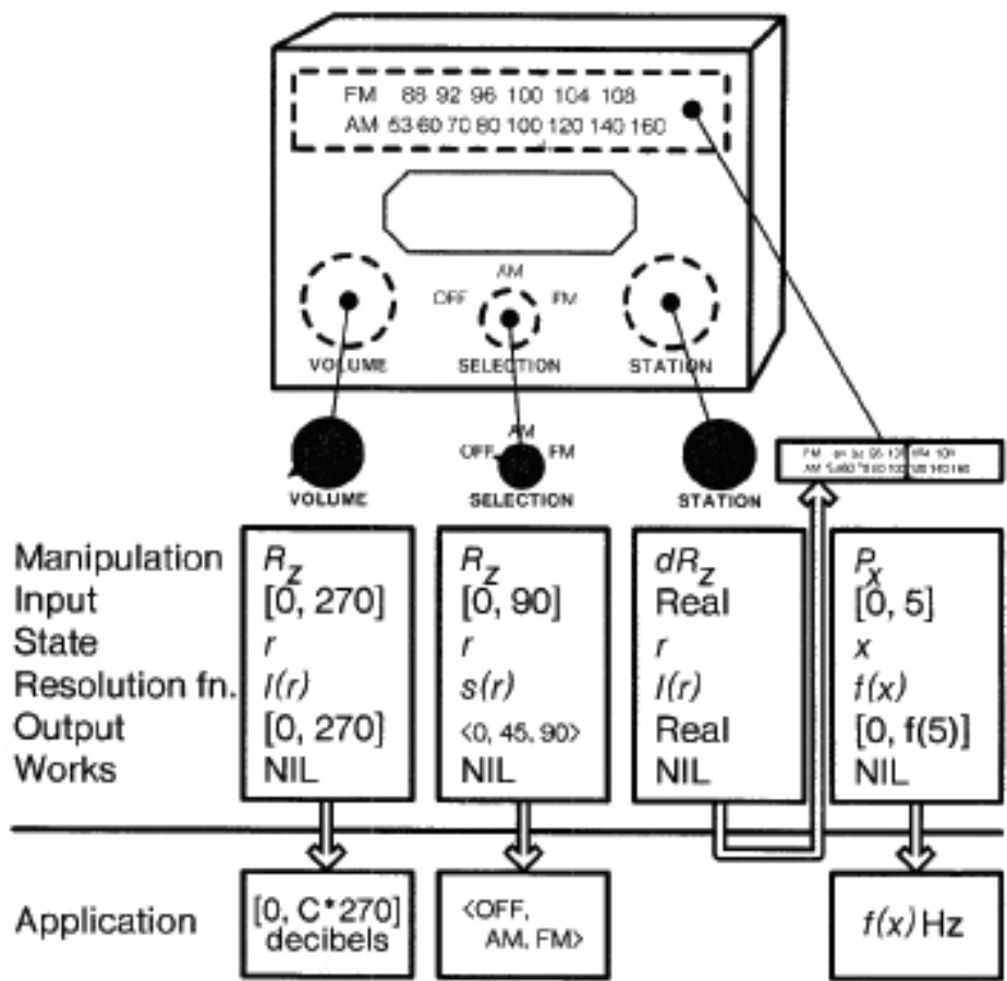
Figure 4.1: Analysis of a simple radio from (Card et al. , 1991). Two rotational devices are connected directly to the application. The third rotational device is connected to a positional device, which is then connected to the application.
