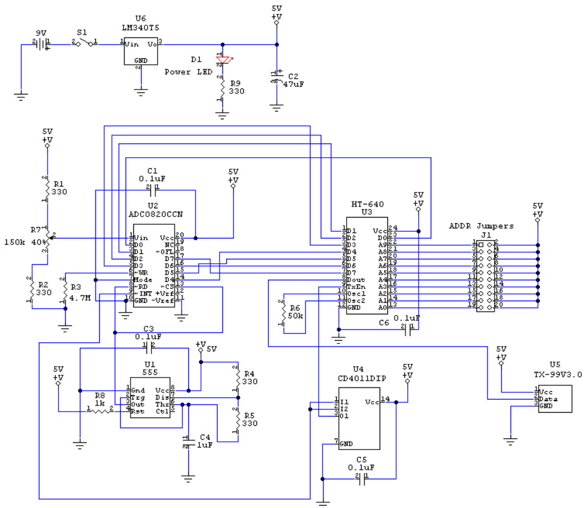
Figure A.3: The circuit diagram for the iSlider.
