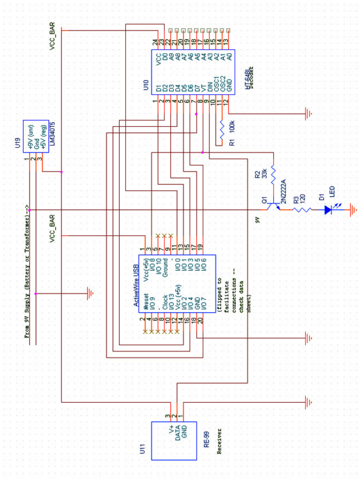
Figure A.4: The circuit diagram for the iStuff proxy receiver.
