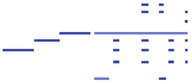
Figure 9. Bars 45–49 of the “Blue Danube” in piano roll notation. The beginning of the theme is still recognizable.
